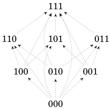
Figure 4.9: Step 1. \leq'_K
