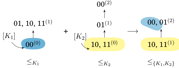
Figure 3.7: Merging two faithful pre-orders using the sum.
