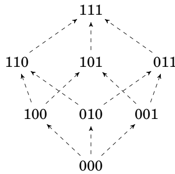
Figure 4.10: Step 2. \leq^*_K
