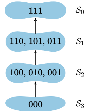
Figure 4.11: Step 3. \leq_K
